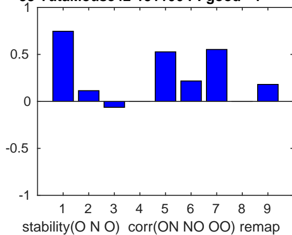
38 YutaMouse42-151106 PFgood= 1
