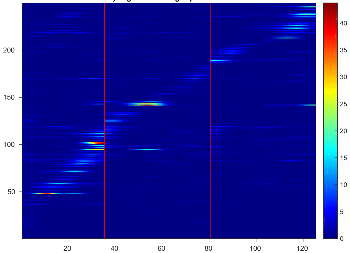
DG a II 5 --sorted--CA3PyrEightMaze-FiringMap--SpeedThreshold--less-lines CA3PyrEightMaze-FiringMap--sorted
