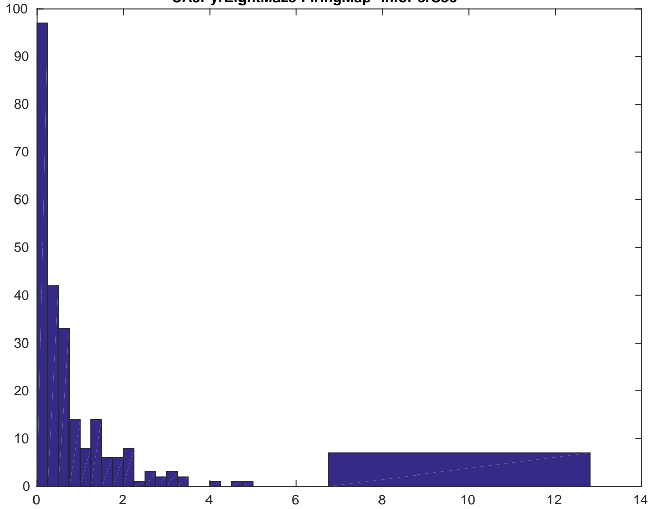
CA3PyrEightMaze-FiringMap--InfoPerSec
