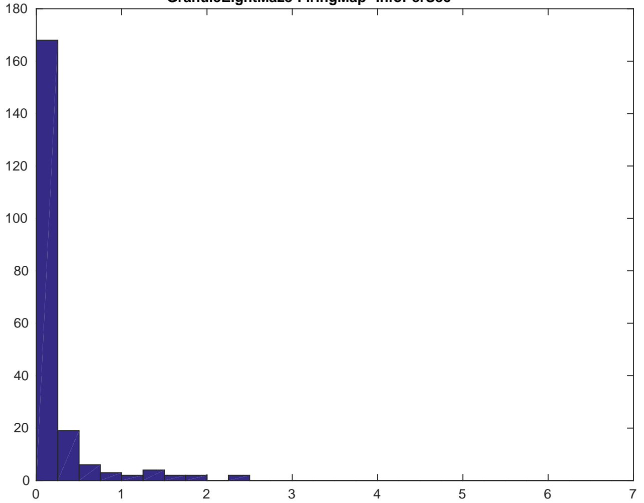
GranuleEightMaze-FiringMap--InfoPerSec
