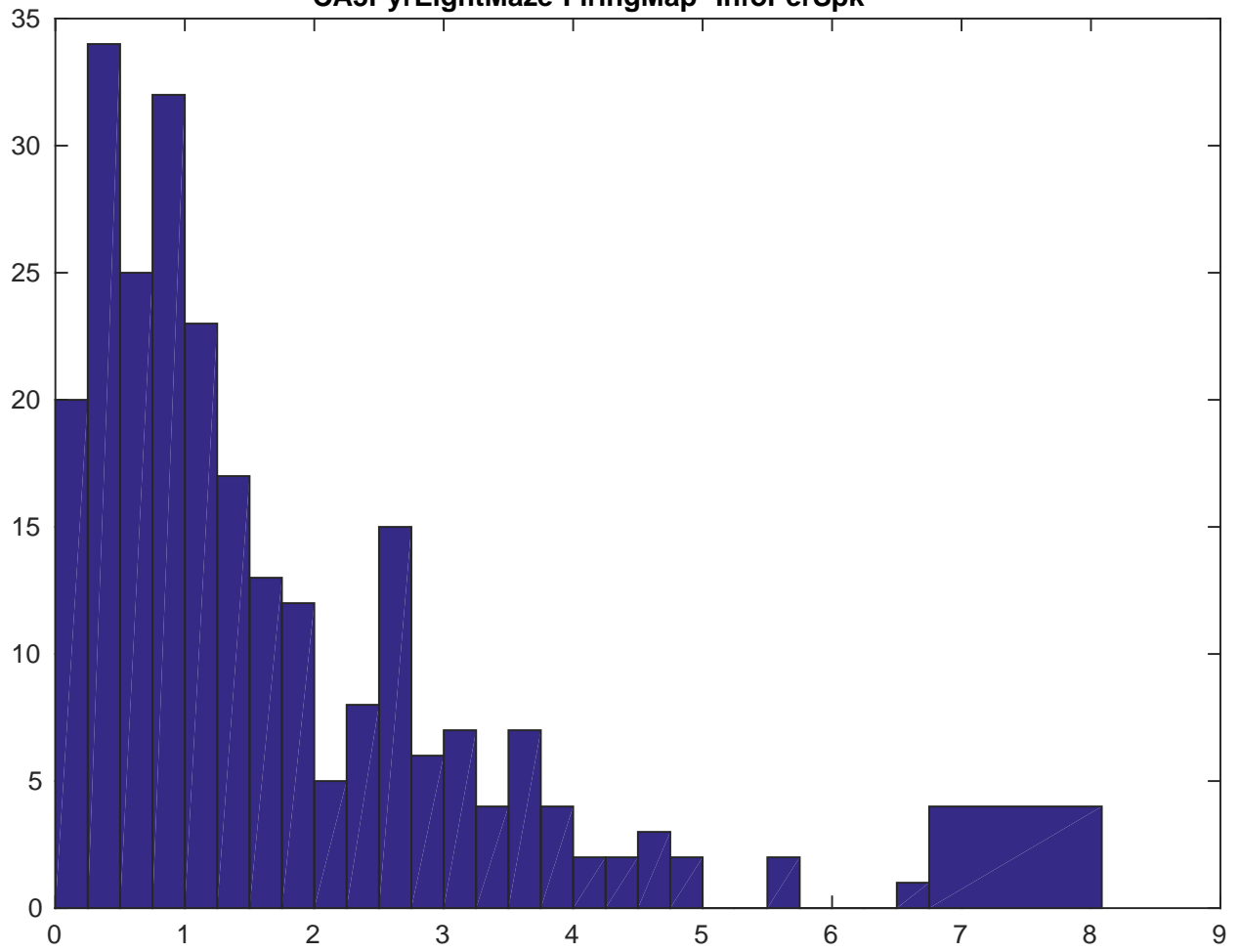
DG a II 5 -2-InfoPerSpk-Dist--nonstim-CA3PyrEightMaze-FiringMap--SpeedThreshold CA3PyrEightMaze-FiringMap--InfoPerSpk
