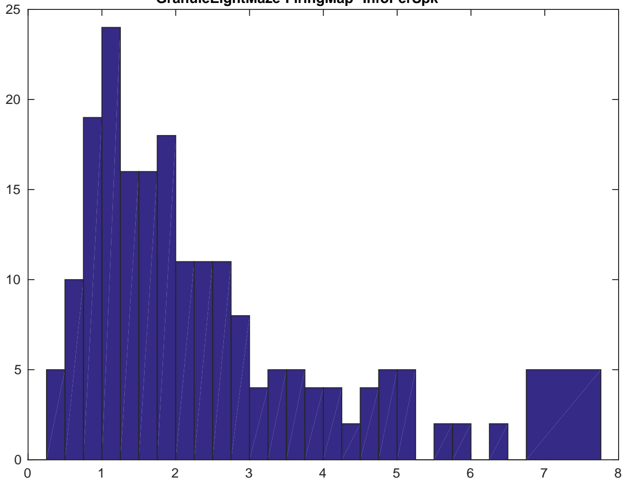
DG a II 5 -2-InfoPerSpk-Dist--nonstim-GranuleEightMaze-FiringMap--SpeedThreshold GranuleEightMaze-FiringMap--InfoPerSpk
