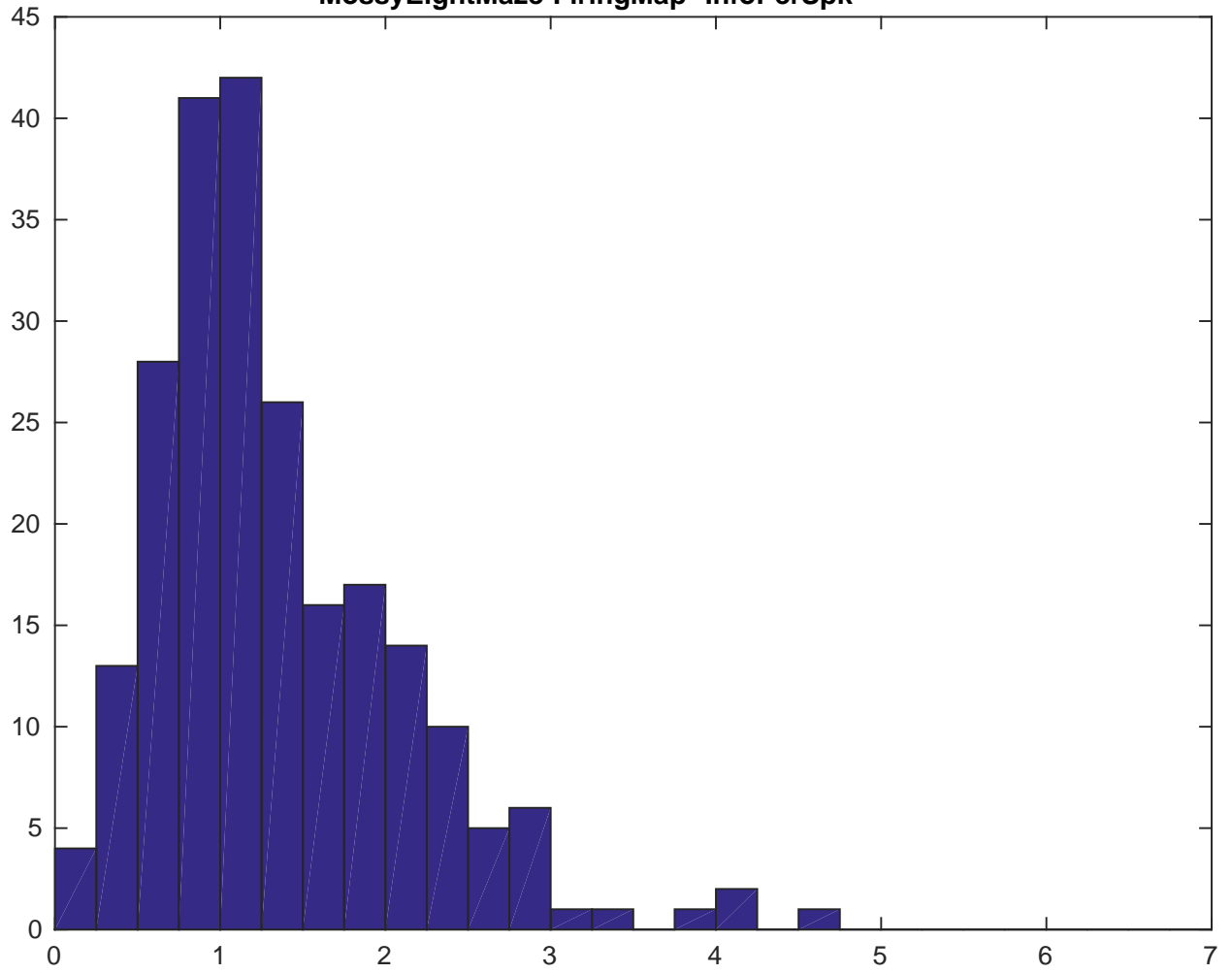
MossyEightMaze-FiringMap--InfoPerSpk
