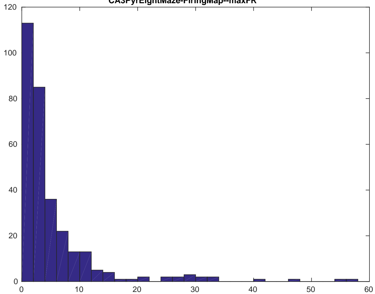
CA3PyrEightMaze-FiringMap--maxFR
