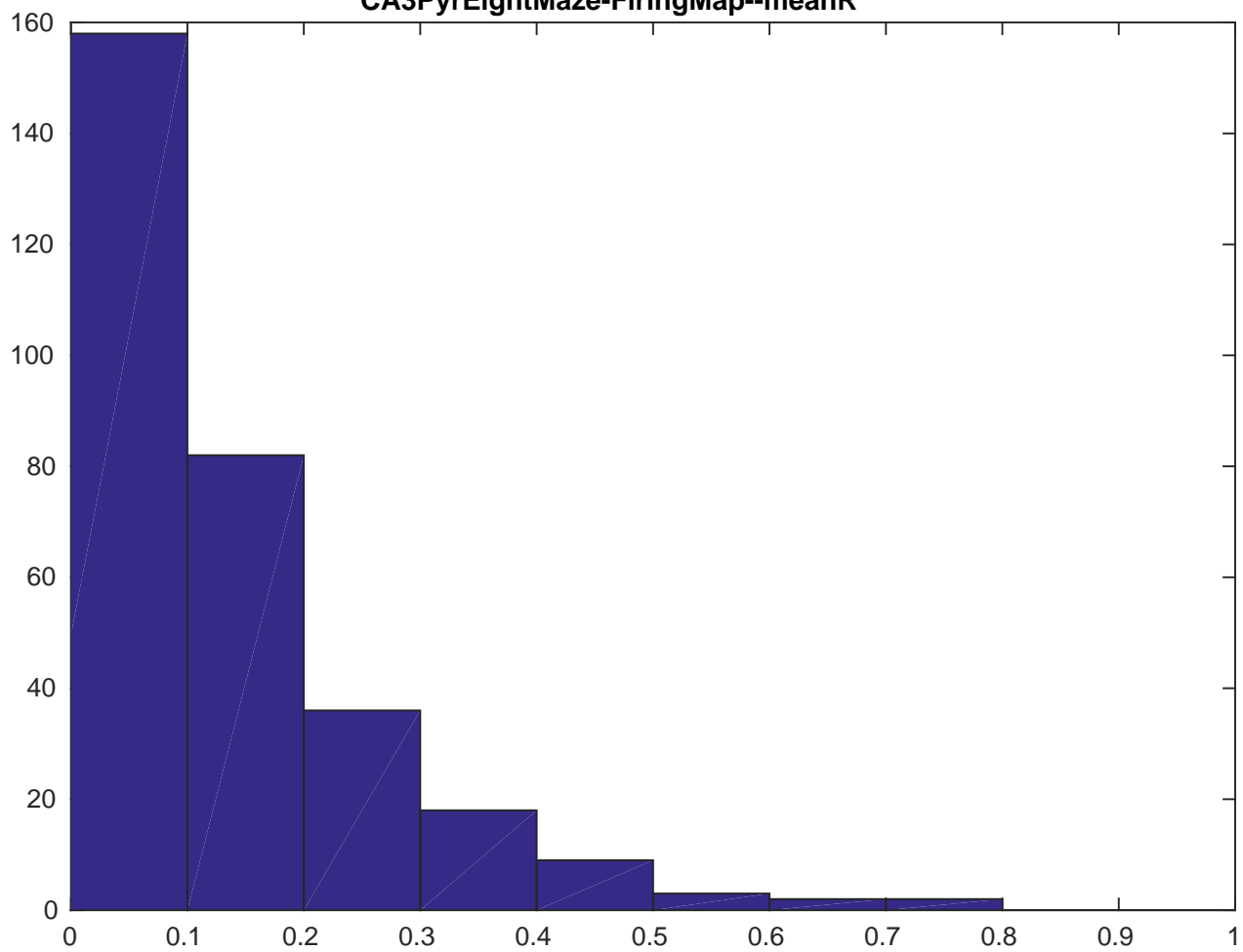
DG a II 5 -2-meanR-Dist--nonstim-CA3PyrEightMaze-FiringMap--SpeedThreshold CA3PyrEightMaze-FiringMap--meanR
