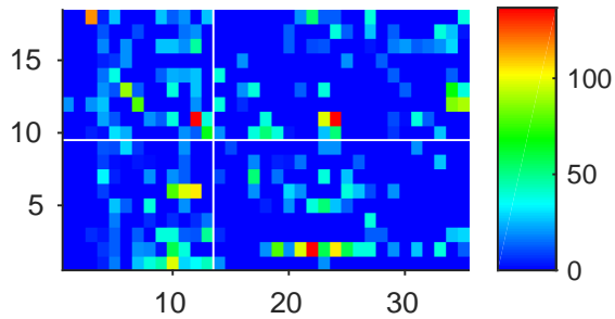
stim p= 0.98795
