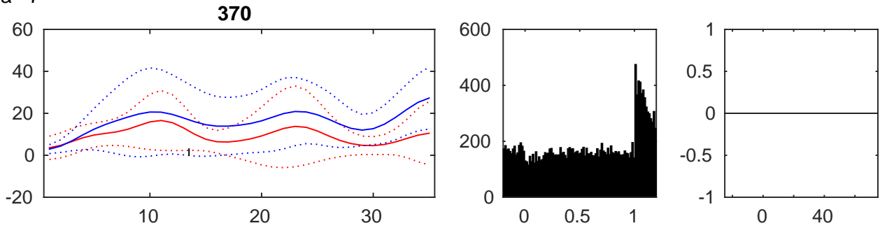
nostimPF:35 StimPF:23
