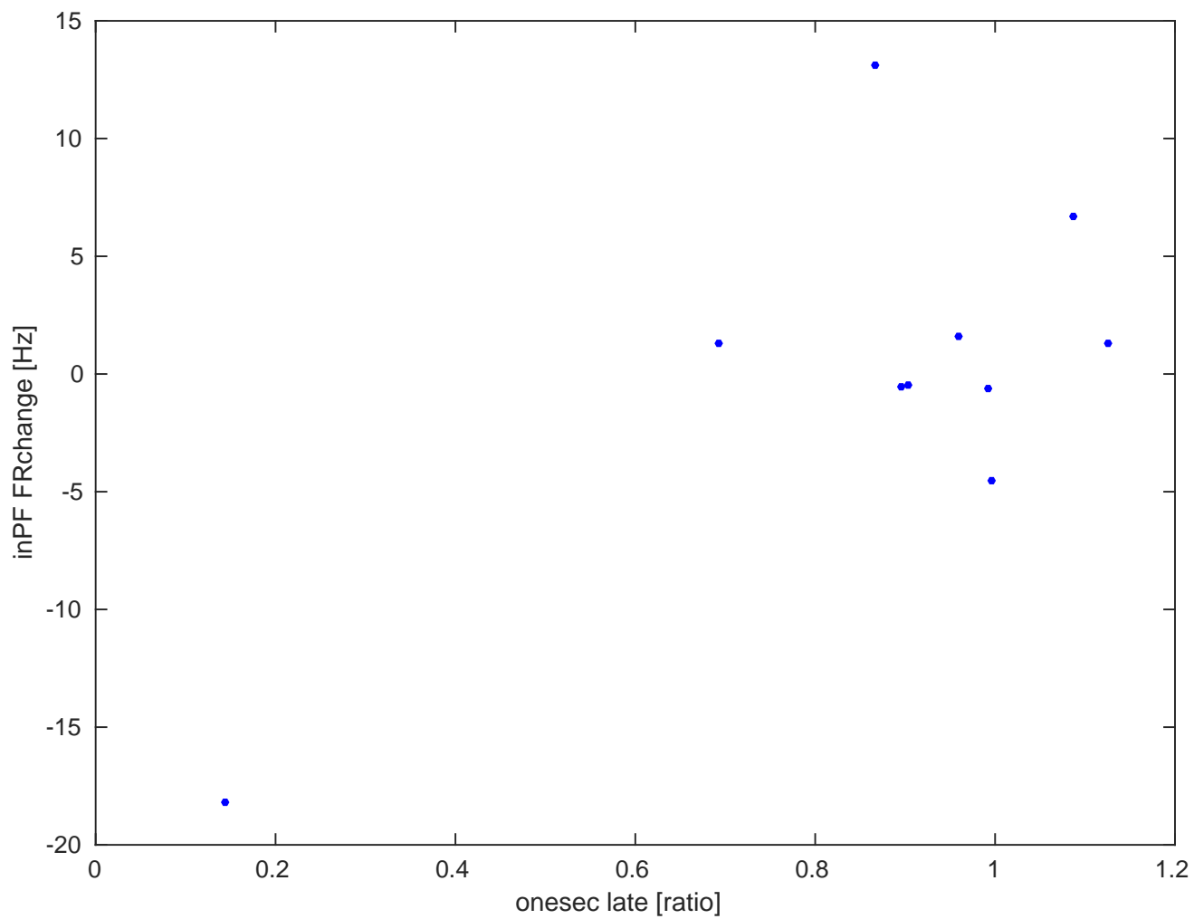
DG a II 7 ---POMC-opto-stim-CA3Pyr--onsecLate-vs-inPF-FRchange
