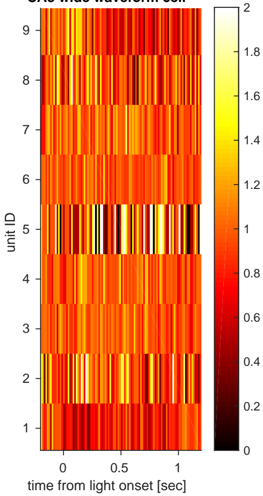
CA3 wide waveform cell
