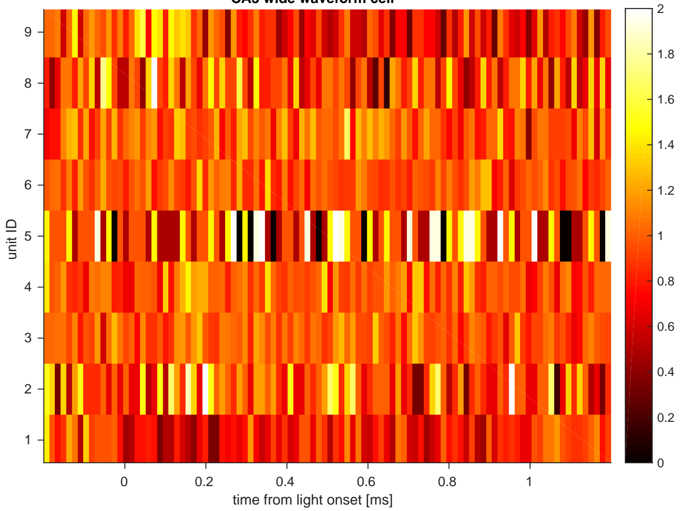
YutaMouse42--CA3 wide waveform cell--1sec CA3 wide waveform cell
