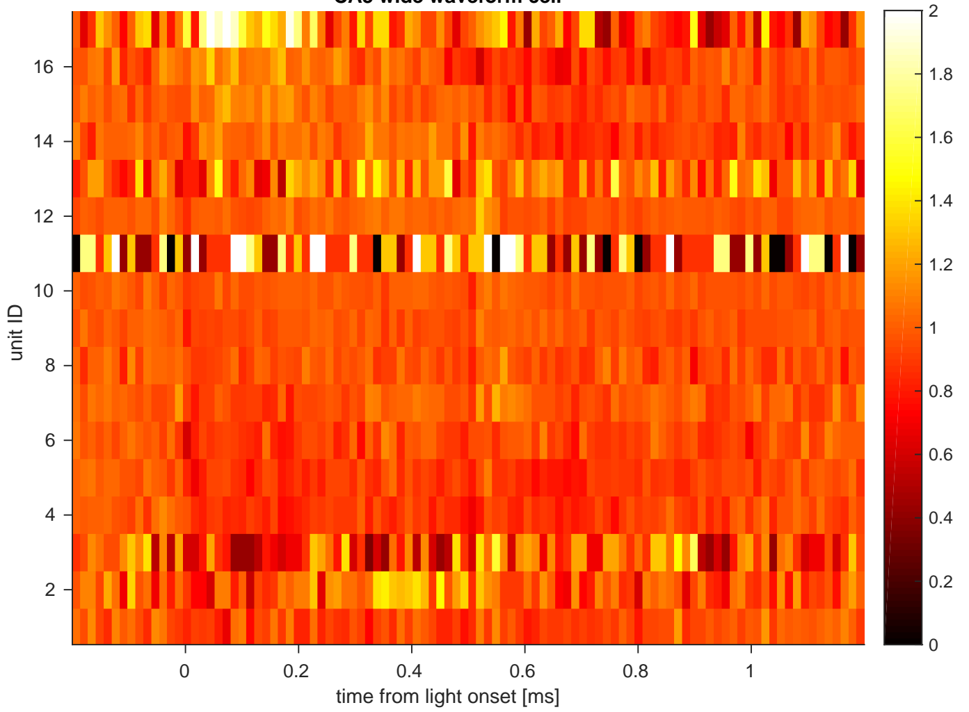
YutaMouse60--CA3 wide waveform cell--1sec CA3 wide waveform cell
