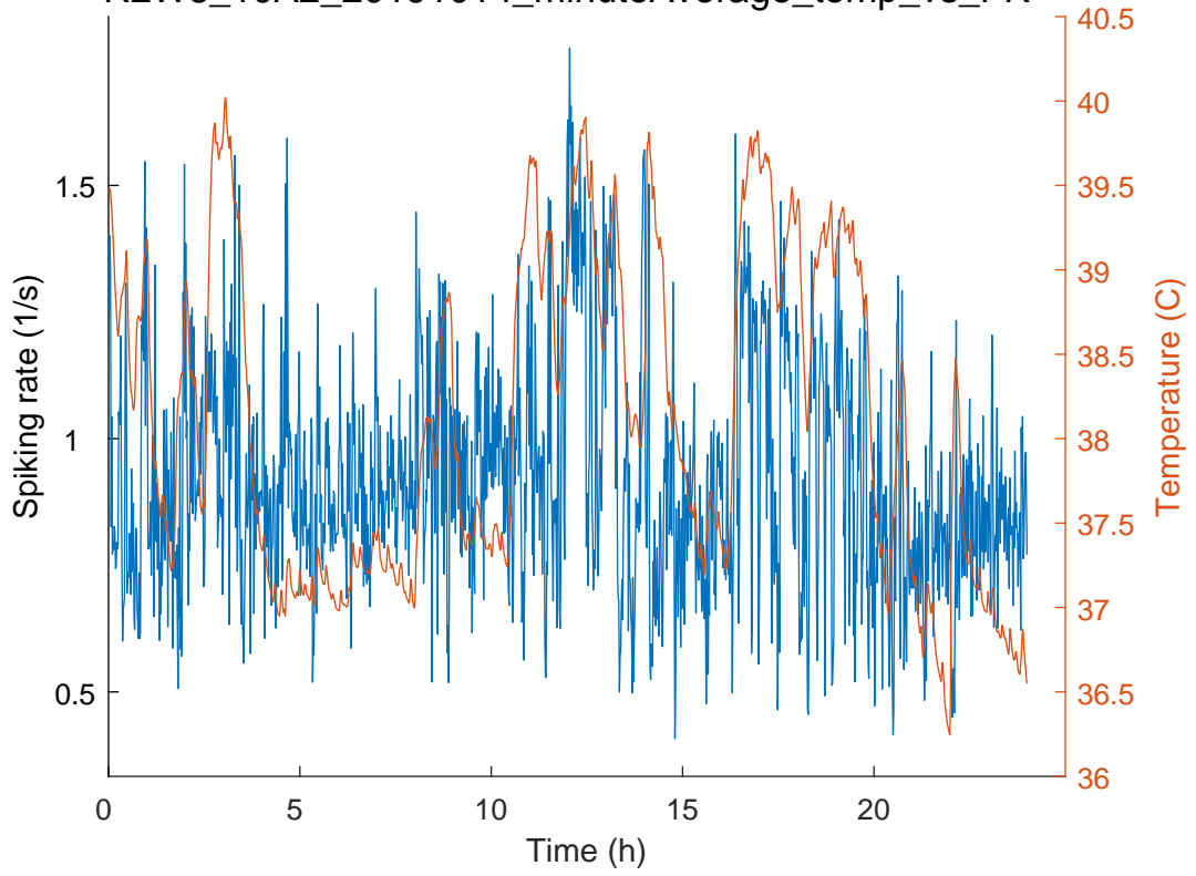
R2W3_10A2_20191014_minuteAverage_temp_vs_FR
