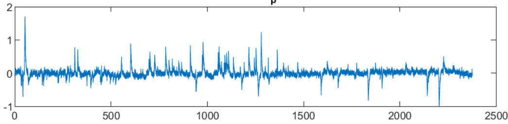
dF/F Response Stim p art12 Cell100
