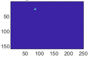
Segment for cell#100
