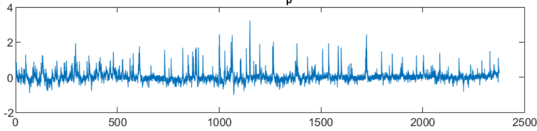
dF/F ResponseStim p art12 Cell102
