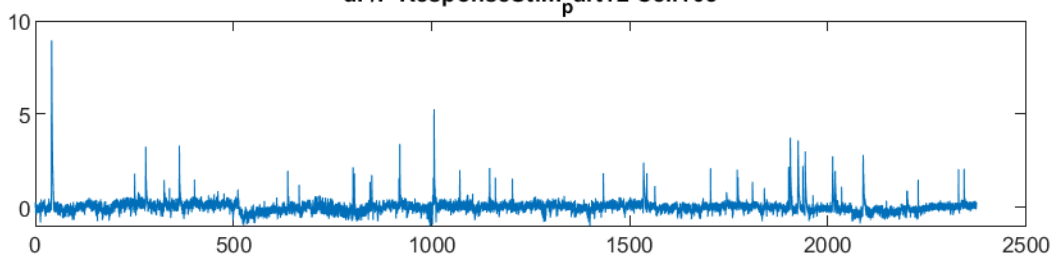
dF/F Response Stim p art12 Cell103
