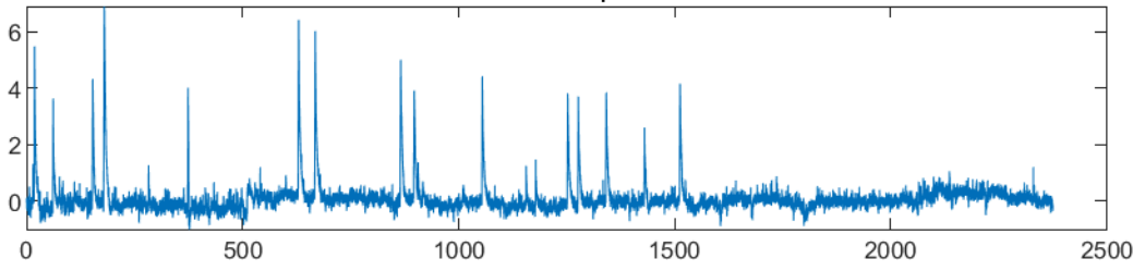
dF/F Response Stim p art12 Cell139
