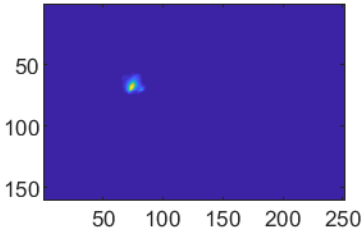
Segment for cell#139
