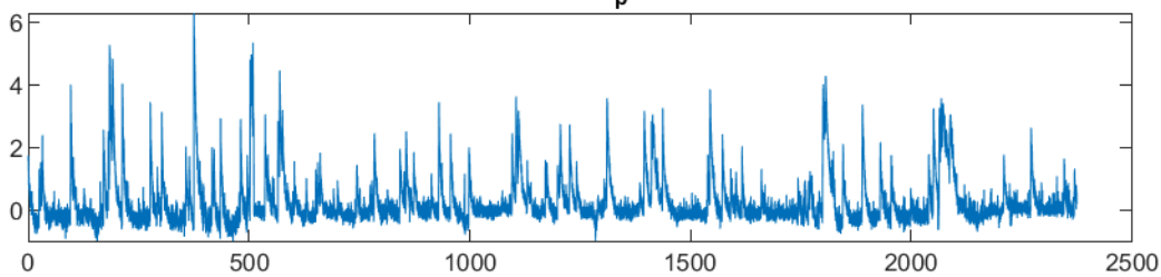
dF/F Response Stim p art12 Cell155
