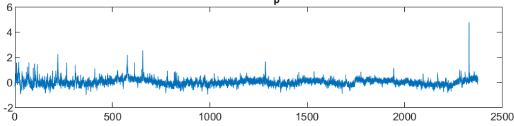
dF/F Response Stim p art12 Cell172
