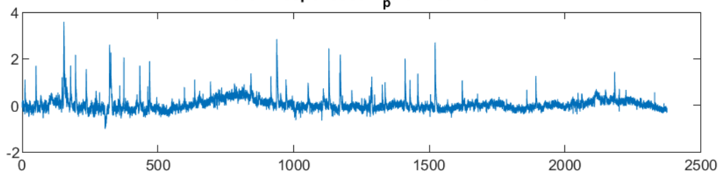
dF/F Response Stim p art12 Cell176
