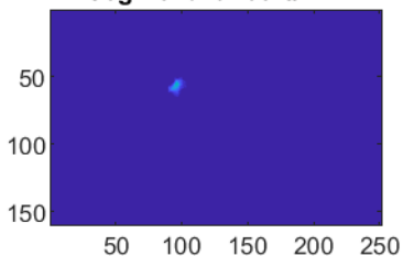
Segment for cell#177
