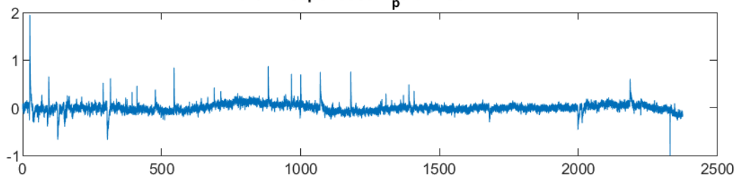
dF/F ResponseStim p art12 Cell177
