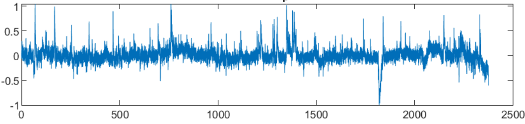
dF/F Response Stim p art12 Cell196
