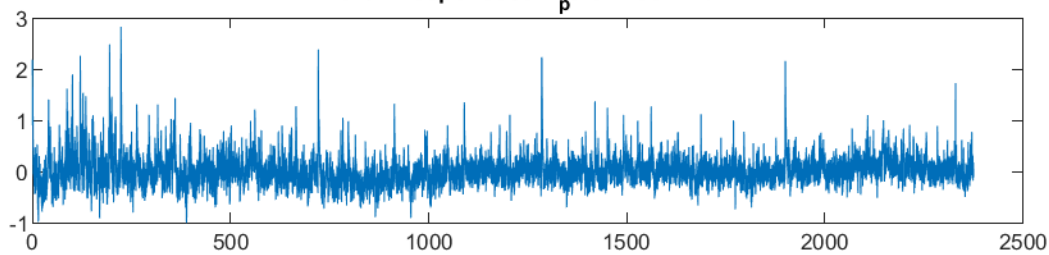
dF/F Response Stim p art12 Cell240
