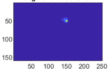
Segment for cell#259
