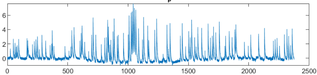
dF/F Response Stim p art12 Cell259
