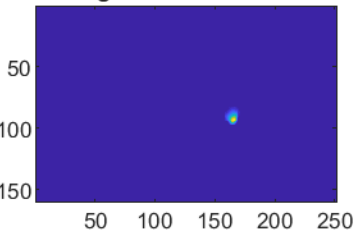
Segment for cell#285
