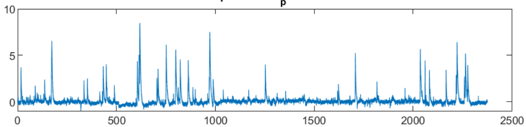
dF/F Response Stim p art12 Cell285
