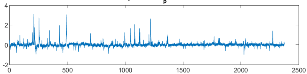
dF/F Response Stim p art12 Cell293
