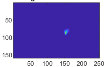
Segment for cell#293
