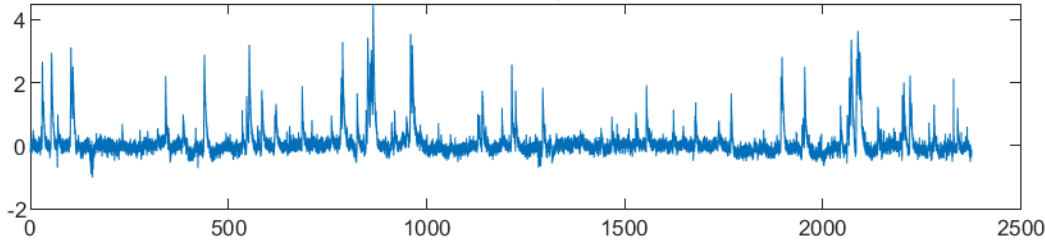
dF/F Response Stim p art12 Cell300
