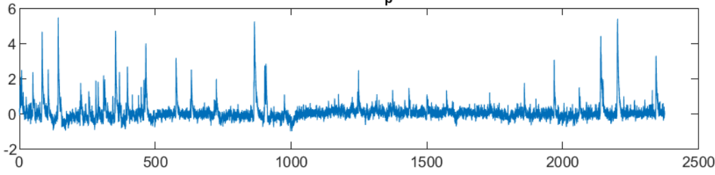
dF/F Response Stim p art12 Cell31
