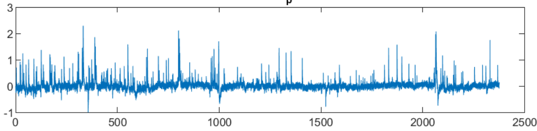
dF/F Response Stim p art12 Cell325
