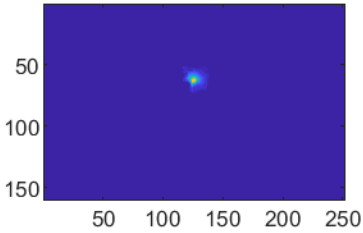
Segment for cell#325
