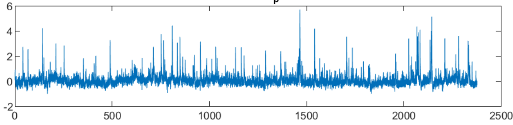
dF/F Response Stim p art12 Cell328
