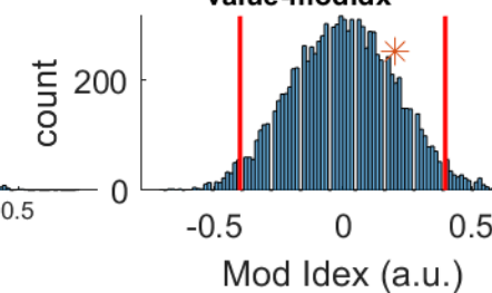
Stim p art12 Spikes Events
