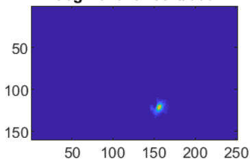
Segment for cell#366
