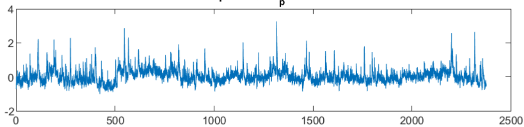
dF/F Response Stim p art12 Cell395
