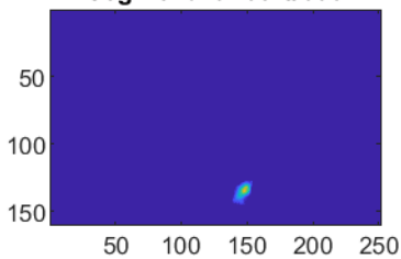
Segment for cell#395
