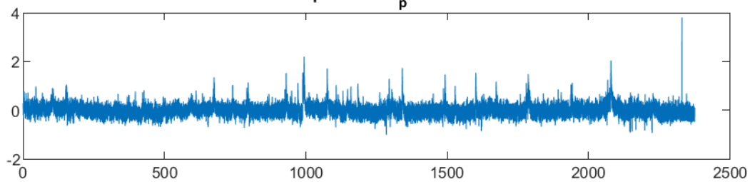
dF/F ResponseStim p art12 Cell437
