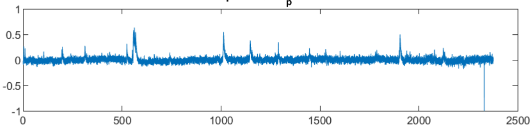
dF/F ResponseStim p art12 Cell444
