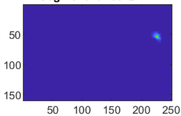
Segment for cell#444
