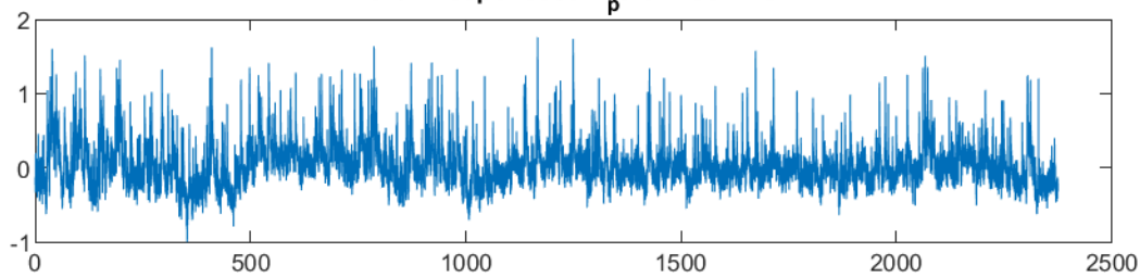
dF/F Response Stim p art12 Cell445
