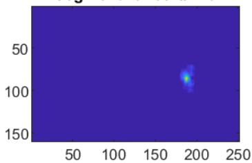
Segment for cell#445
