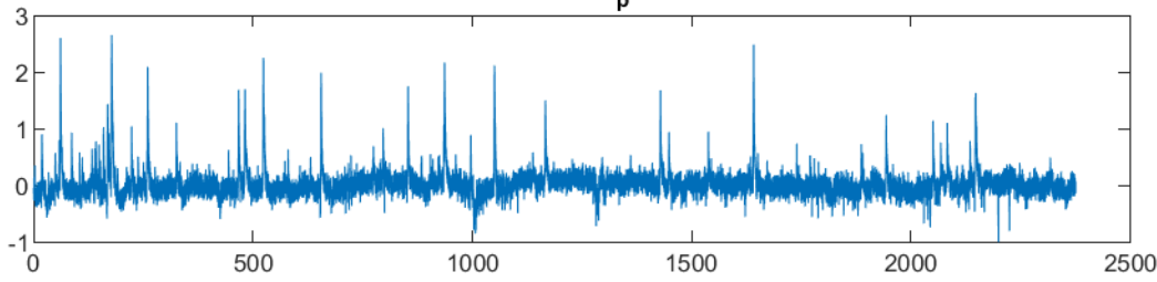
dF/F ResponseStim_p_art12 Cell481
