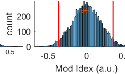
Stim_p_art12 Spikes Events Shuffle modix per trial
