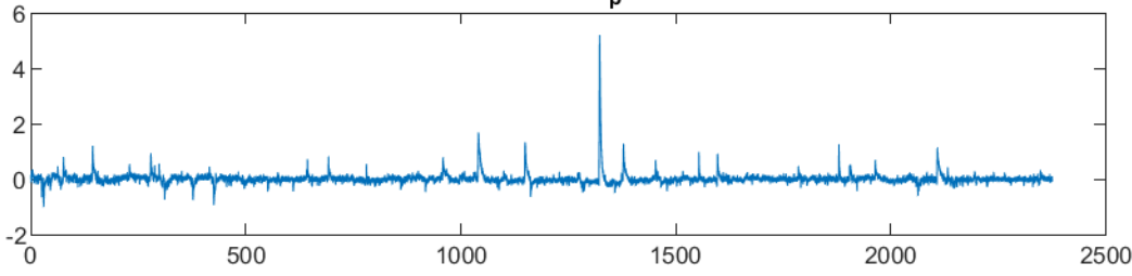
dF/F Response Stim_p_art12 Cell63
