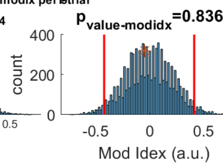
Stim_p_art12 Spikes Events
