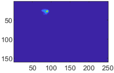
Segment for cell#73
