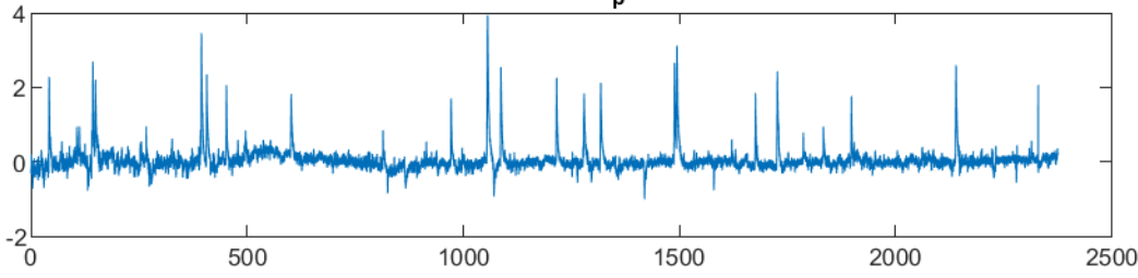
dF/F Response Stim_p_art12 Cell73
