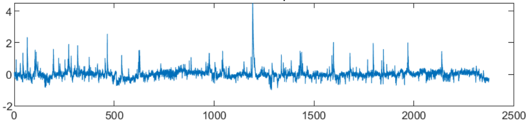
dF/F Response Stim_p_art12 Cell75
