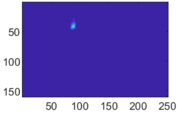
Segment for cell#75
