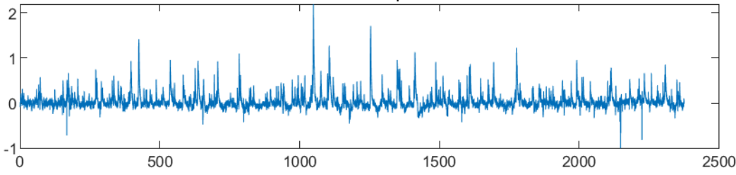
dF/F Response Stim_p_art12 Cell76
