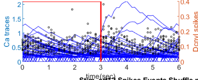
Stim_p_art12 Spikes Events Shuffle modix per trial
