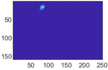
Segment for cell#76
