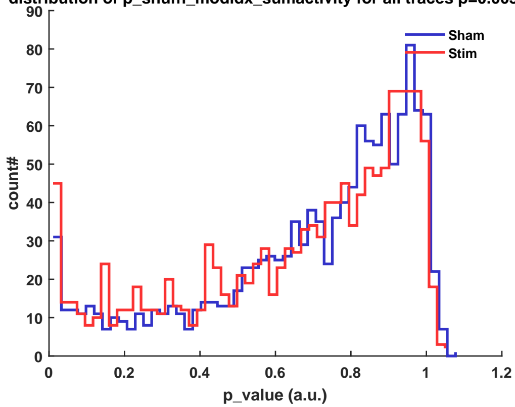
distribution of p_shuffl_modidx_sumactivity for all traces p=0.003314
